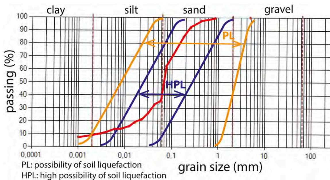
FIGURE 12 Grain size curve (red line) of sample taken in the historical or protohistoric alluvial deposit (units 2a and 2b) at 1.40–1.60 m below ground level in the borehole S2 (Figure 9). HPL: high possibility of soil liquefaction; PL: possibility of soil liquefaction (Sherif et al., 1977).
