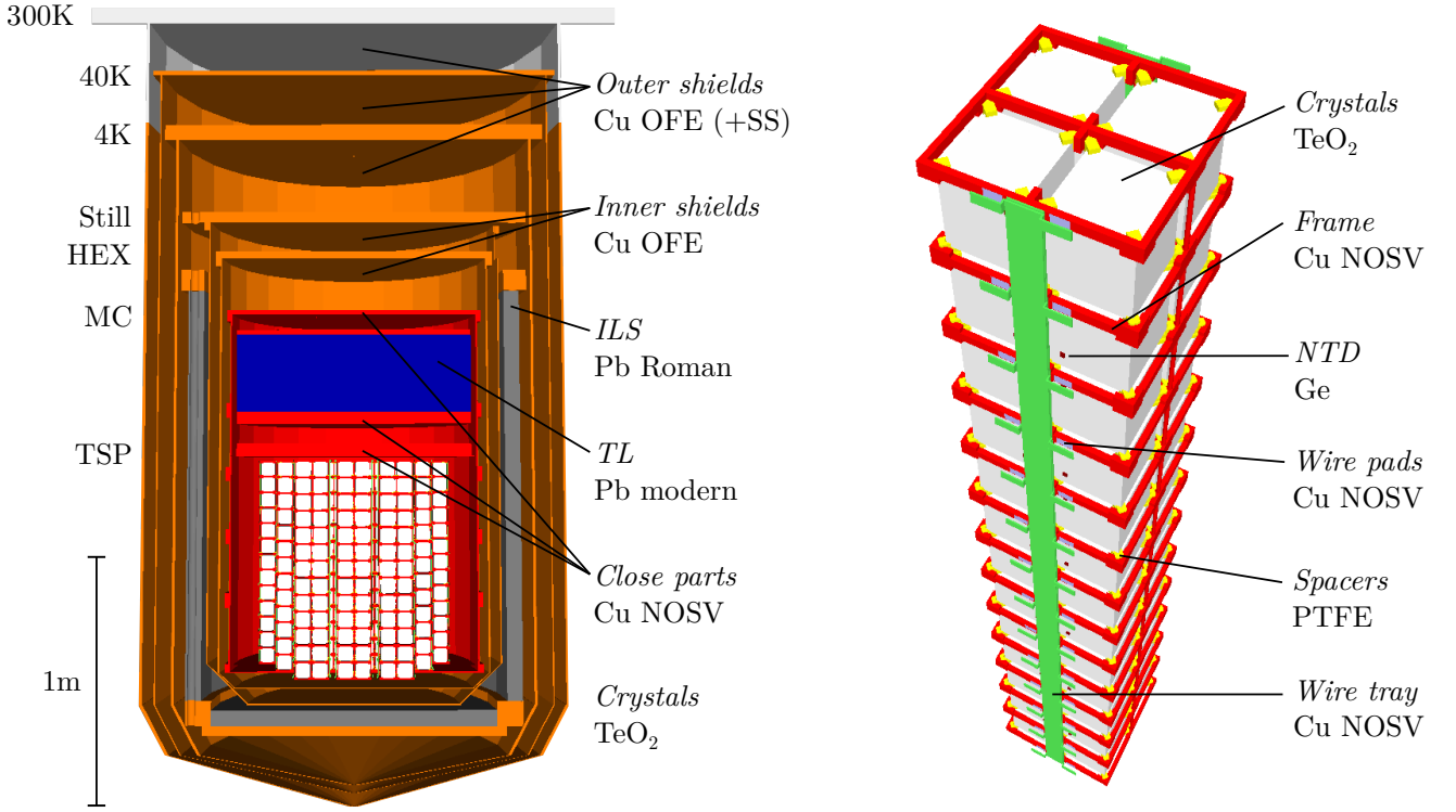
FIG. 1. (Left) Rendering of the CUORE cryostat and detector as implemented in the Monte Carlo simulation; the actual length scale is reported as a reference. On the left, the different thermal stages are reported; on the right, the volumes are presented as grouped in the Monte Carlo, together with the material they are made of. The \text{TeO}_2 crystals are depicted in white, the NOSV copper components in red, the OFE copper in orange, the TL in blue, the ILS in gray and the 300K stainless steel in light gray. (Right) Detailed view of a CUORE tower, where all the different components are showed in different colors: \text{TeO}_2 crystals in white, NOSV-copper frames in red, PTFE supports in yellow, NOSV-copper wire trays in green and NOSV-copper wire pads in blue.
