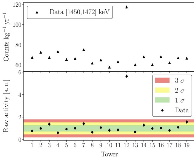
FIG. 8. (Top) Yield normalized by the exposure for the potassium 1461-keV line of ^{40}\text{K} for the 19 towers of CUORE. Tower 12 contains approximately double the events compared to the other towers. (Bottom) Normalization factor of the ^{40}\text{K} contamination in the Crystals bulk when performing the fit on the towers individually. The colored bands refer to the 1, 2 and 3 standard deviations coming from the activity distribution when considering all the towers except tower 12.
