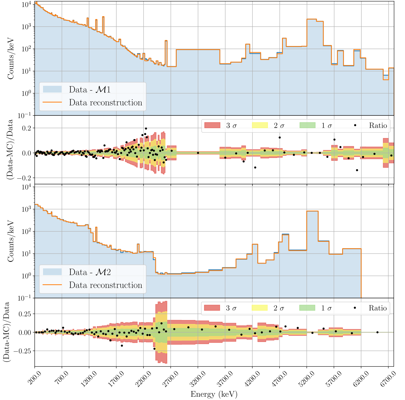
FIG. 4. ( Top panels ) Reconstruction of the \mathcal{M}1 events and residuals. ( Bottom panels ) Cumulative spectrum of the individual \mathcal{M}2 events and residuals. The residuals are quoted as fractions of data, with the statistical uncertainties represented as 1\sigma , 2\sigma and 3\sigma standard-deviation bands. The \mathcal{M}2 spectrum ends at 6200 keV because this is the maximum energy for the events in the highest total-energy band taken into account.
