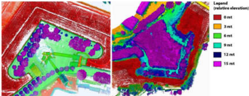
Fig. 7 – Comparison of DSM of Santa Croce (on the left) and Santa Cristina on the right. (Source: created by the authors)
