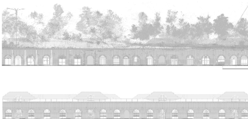
Fig. 4 - Forte Monte Mario. The elevation of the troop quarters, showing the current state and a reconstruction of its original condition. Source: drawings by Lucia Chiarotti, Giulia Lamolinara, and Chiara Middei (graduation laboratory).
