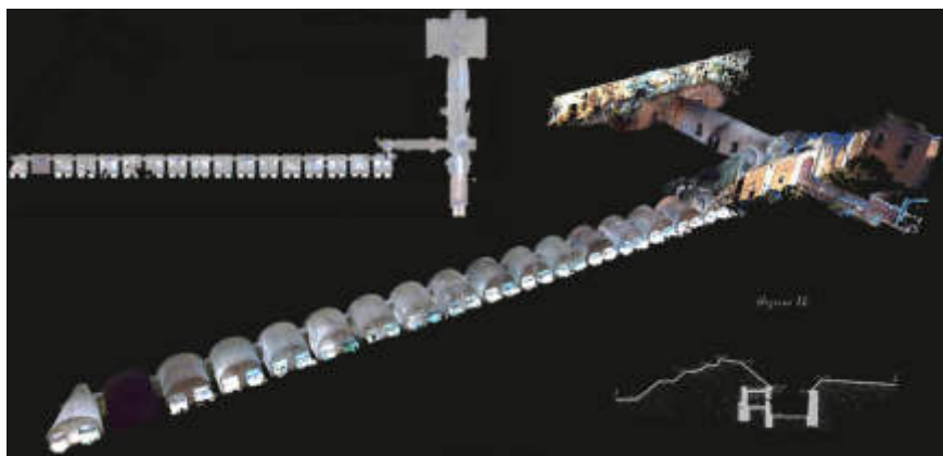
Fig. 7 - Fort Monte Antenne. Top left: plan of the rifle galleries with the location of the targets. Center: point cloud obtained through dynamic SLAM. Bottom right: section of the rifle galleries from the drawing preserved at ISCAG. Source: created by the authors.
