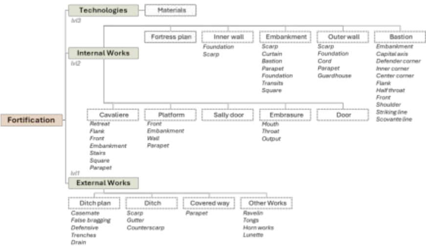
Fig. 2 - Hierarchical classification of fortification components (WBS), organized into External Works, Internal Works, and Technologies. Source: created by the authors.
