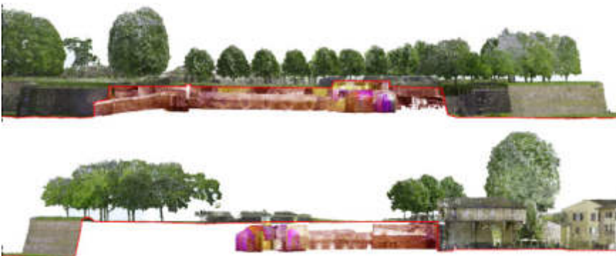
Fig. 5 – Two sections of Santa Croce baluard with tunnel area highlighted in red. (Source: created by the authors)
