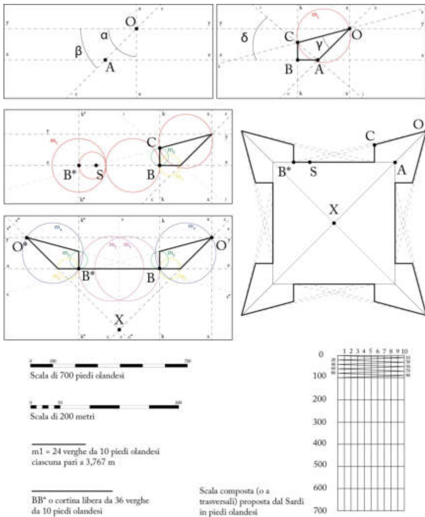
Fig. 4 - Geometric construction of the defended polygon from the third book of the Corno Dogale by Pietro Sardi (Source: Rechichi, 2024; Elaborated by Rechichi, P.)
