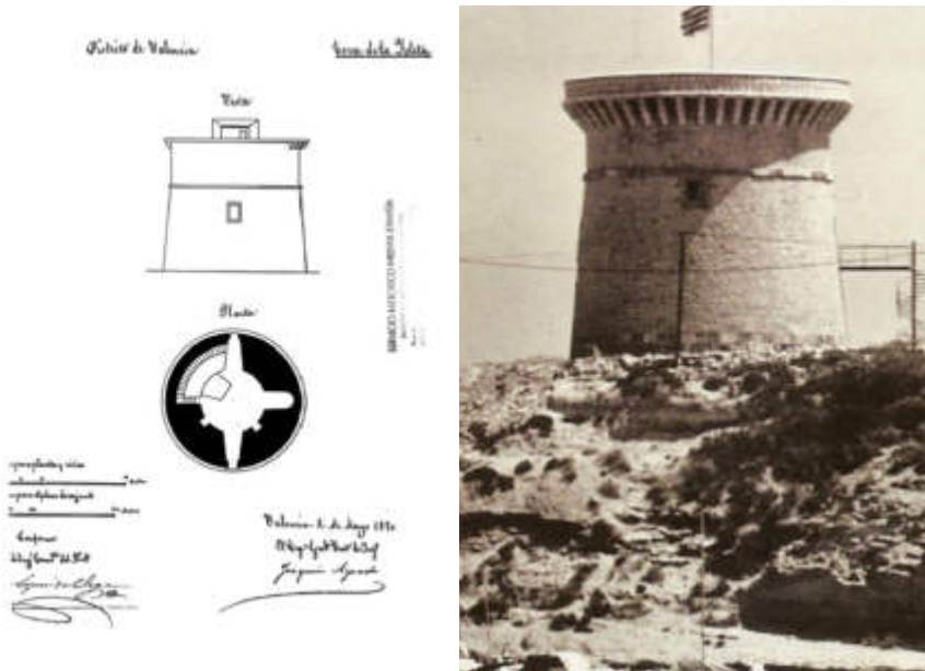
Fig. 4 - Floor plan and elevation of the Isleta Tower. Aguado Report, 1870 (left). Tower after restoration (right). Open source.
