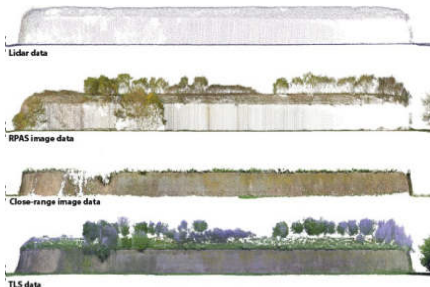
Fig. 6 – Comparison of the same wall of Santa Cristina baluard with different 3D survey techniques. (Source: created by the authors)
