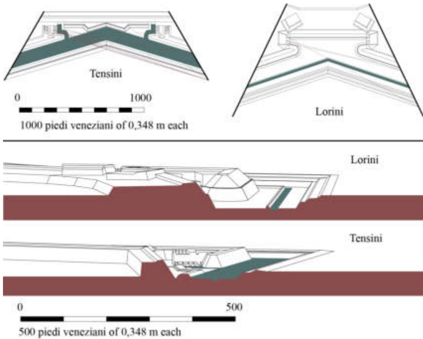
Fig. 8 - Critical redrawing of icnographic projections of fortificatory systems from the treatises by Bonaiuto Lorini and Francesco Tensini. Perspective sections of the same fortificatory sytems (Source: Rechichi, 2025; Elaborated by Rechichi, P.)
