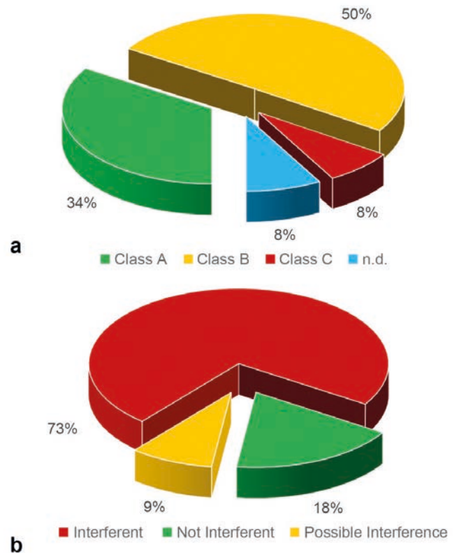
FIG. 4 - a) Percentage distribution of volume classes of the ground effects inventoried. b) Percentage distribution of interaction between the ground effects and the main infrastructures.
