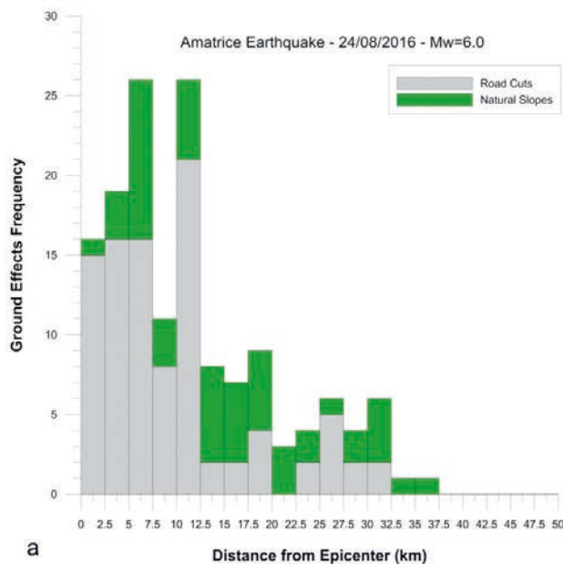
FIG. 12 - Distribution of ground effects triggered by the 24 th August 2016 M_w 6.0 earthquake with epicentral distance (a) distinguishing occurrence on natural slopes and on man-made cuts (b).
