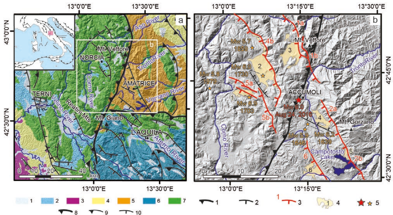
FIG. 1 - a) Simplified geological map of the study area; 1 continental Pleistocene-Holocene deposits; 2 continental Villafranchian deposits; 3 Pleistocene volcanic products; 4 Plio-Pleistocene marine sediments; 5 Tortonian-Messinian terrigenous deposits; 6 Triassic-Miocene Latium-Abruzzo platform limestones and dolomites; 7 Triassic-Miocene Umbria-Marche pelagic limestones and marls; 8 major thrust front; 9 thrust fault; 10 normal fault. b) 24 th August 2016 ( M_w 6.0) earthquake epicentral area; 1 major thrust front; 2 normal fault; 3 active normal fault (1a: Mt. Bove fault, 1b: Mt. Vettore fault, 2a: Mt. Gorzano fault, 2b: Campotosto fault, 4b: Notoria-Mt. Pizzuto fault, 5a: Cascia fault, 5b: Castel S.Maria-Cittareale fault, 6: Montereale fault); 4 intermontane basin (1: Cascia Plain, 2: Norcia Plain, 3: Castelluccio Plain, 4: Amatrice Plain, 5: Campotosto Plain, 6: Montereale Plain); 5: earthquake epicenters.
