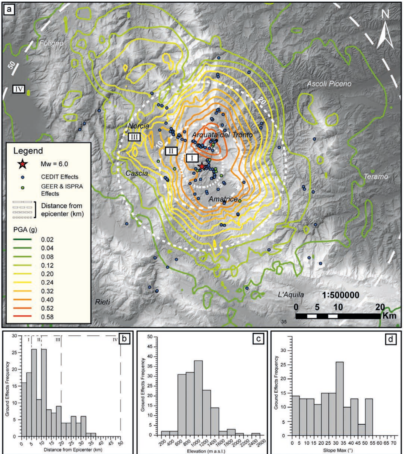
FIG. 11 - Distribution of triggered ground effects after the 24 th August 2016 M_w 6.0 earthquake. a) shaking map (from INGV – http://shakemap.rm.ingv.it/ ) and inventoried ground effects (location of mainshock epicenter is also reported). Further ground effects reported by GEER and ISPRA working groups are also shown; b) earthquake-triggered ground effects distribution vs. epicentral distance; c) earthquake-triggered ground effects distribution vs. elevation; d) earthquake-triggered ground effects distribution vs. maximum slope (Zevenbergen & Thorne, 1987).
