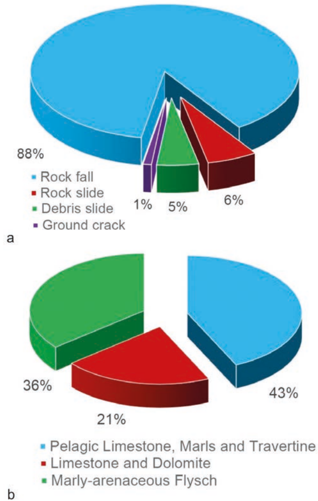
FIG. 9 - Percentage distribution of: a) landslide typology; b) involved lithological classes.
