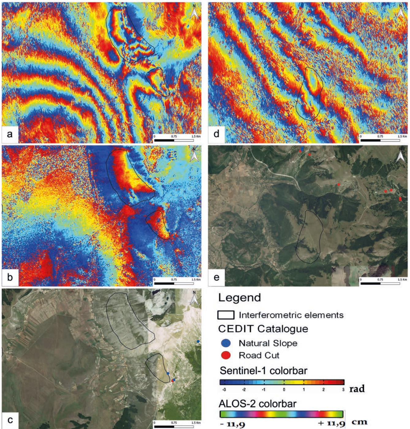
FIG. 5 - Ground effects inventoried by interferometric satellite images from Sentinel-1 (a) and ALOS-2 (b) images. Polygons 1 and 2 enveloping the deformation effects are compared with the field inventoried ground effects (c). Ground effects inventoried by interferometric satellite images from Sentinel-1 (d) images. The polygon 3 enveloping the deformation effects are compared with the field inventoried ground effects (e).
