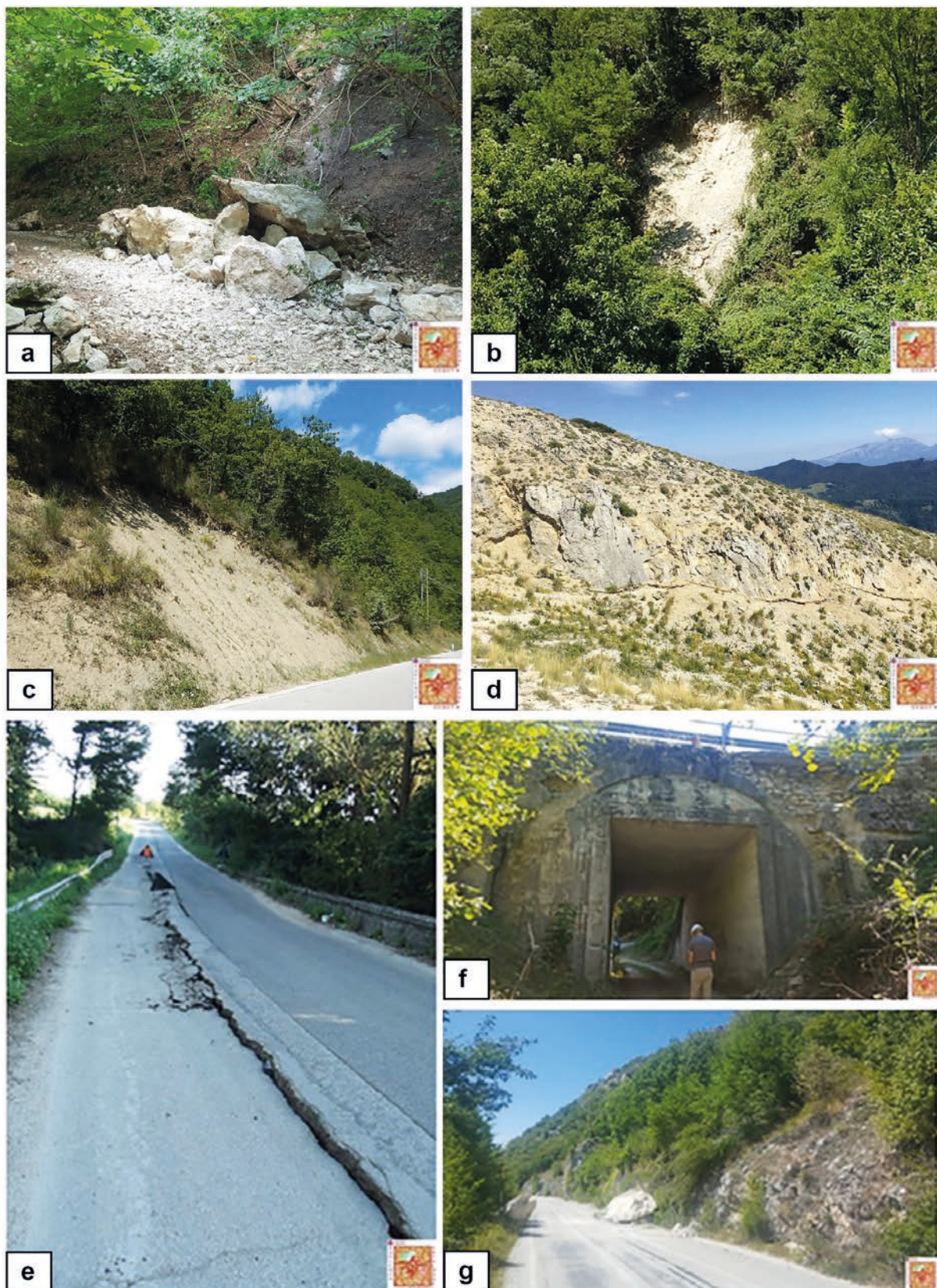
FIG. 3 - Examples of inventoried ground effects: rock fall (a); rock slide (b); debris slide (c); ground crack (d). Examples of ground effects interacting with infrastructures and lifelines: ground crack due to a landslide observed along a roadway (e); structural damages of a bridge (f); rock block on a roadway (g).
