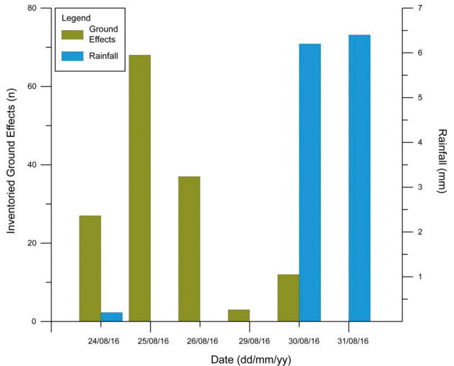
FIG. 2 - Time schedule of field works, with the number of ground effects inventoried for day and the cumulative daily rainfall.
