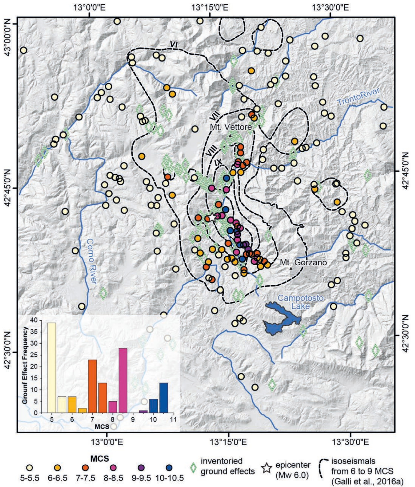
FIG. 10 - Macroseismic field from Galli & alii (2016a, 2016b) and distribution of ground effect frequency vs. MCS local intensity.
