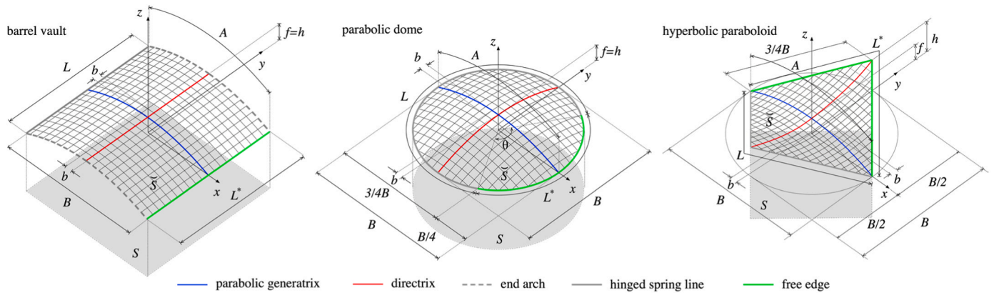
Fig. 1. FreeGrid DBGs: barrel vault, parabolic dome, hyperbolic paraboloid.
