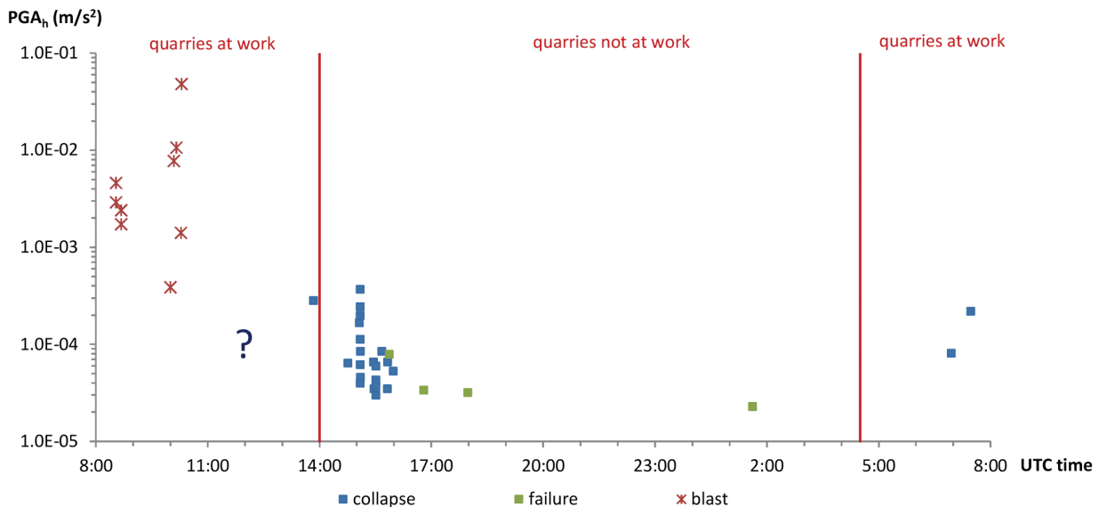
Fig. 12 - Time vs. PGA_n for the events recorded in the 26-27 July 2013 measurement campaigns; the question point indicates a period in which occurrence of gravity-induced slope instability events could be nor excluded neither confirmed because of their signals in the superonogram may have been masked by vibration related to the quarry working equipment
