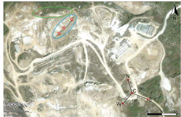
Fig. 2 - Satellite view showing the SNS array installed in the quarry district of Coreno Ausonio: the “reference wall” is shown by the green ellipse, the “reference quarry” by the blue ellipse and the blasts of known location by the red stars
