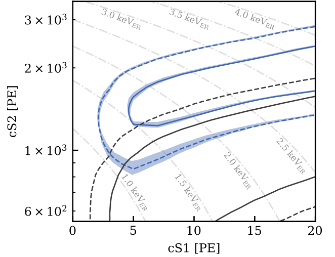
FIG. 6. Shape uncertainty of the ER model constrained by the ^{220}\text{Rn} calibration data. The blue (gray) solid and dashed lines represent the contours of the ER background ( 200 \text{ GeV}/c^2 WIMP) containing 68% and 95% of expected events in the ROI. The transparent blue regions show the shape uncertainty by varying the two shape nuisance parameters by \pm 1\sigma . Dash-dotted lines are contours of constant ER-equivalent energy in units of \text{keV}_{\text{ER}} .
