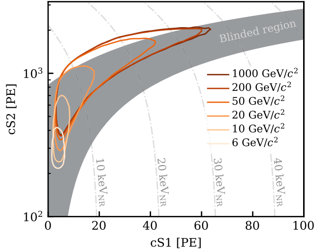
FIG. 5. Expected distribution in cS1 – cS2 space from spin-independent WIMP nuclear recoil for WIMP masses from 6 \text{ GeV}/c^2 to 1000 \text{ GeV}/c^2 . The contours contain 68% of expected events in the ROI. The blinded region, which is exclusively applied to the WIMP search dataset, is shown for reference as a gray band, and dash-dotted lines are constant NR-equivalent energy contours.
