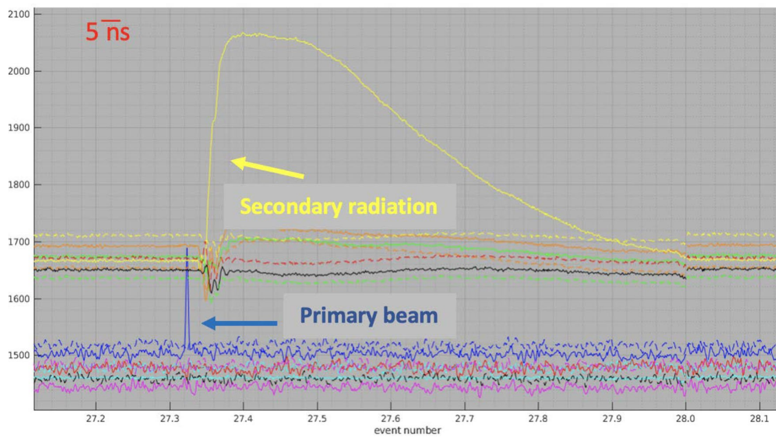
Fig. 36 Example of a coincidence between the signals corresponding to a primary beam proton crossing the silicon beam monitor (blue) and a prompt photon detected by an I3-PET LFS scintillator module (yellow)
