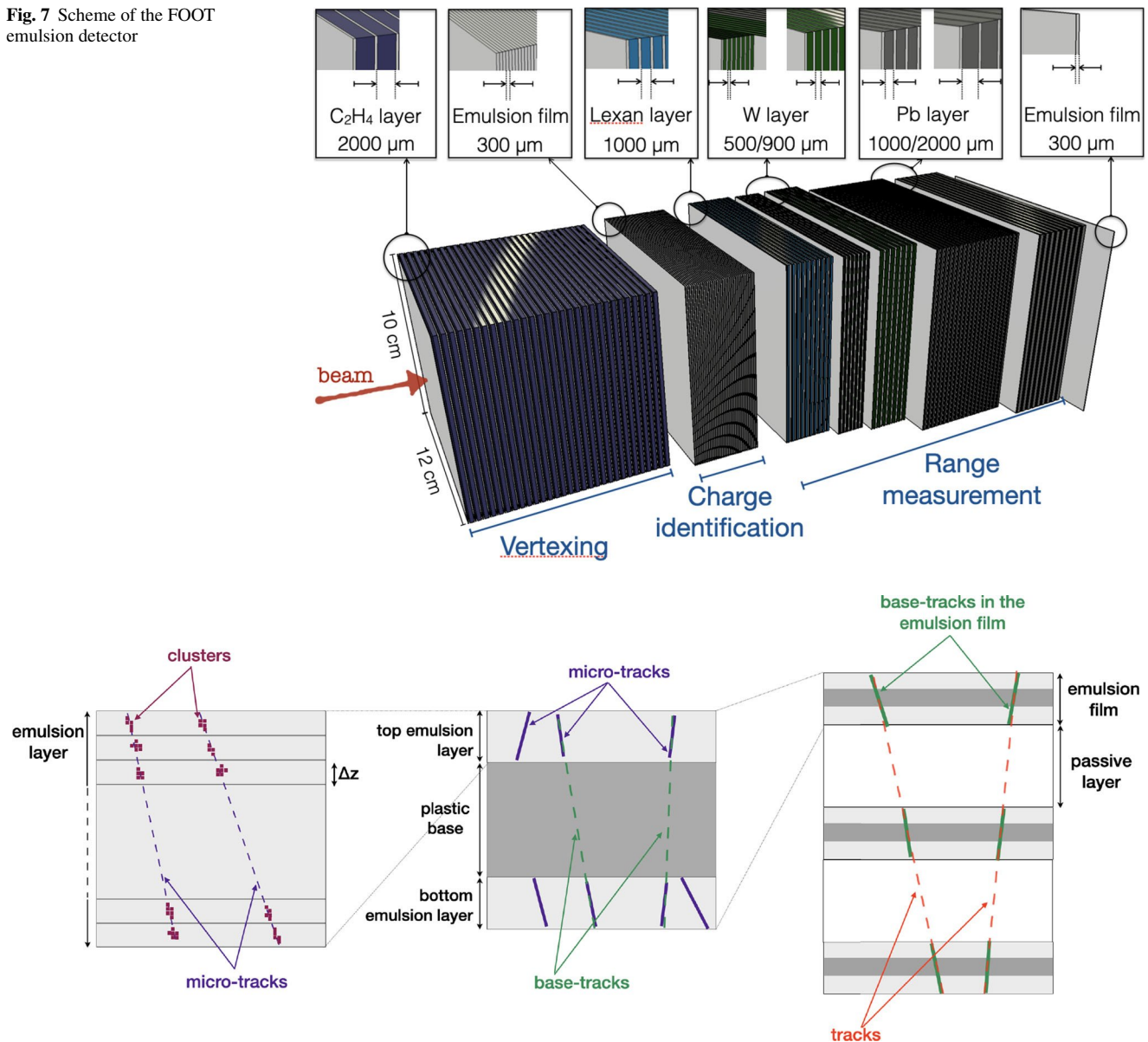
Fig. 8 Schematic drawing of a tracks reconstruction: different tomographic images, grabbed at equally spaced depth levels through the sensitive layer (left), micro-tracks association between two emulsion layers to form a base-tracks (center) and base-tracks association to form a track
