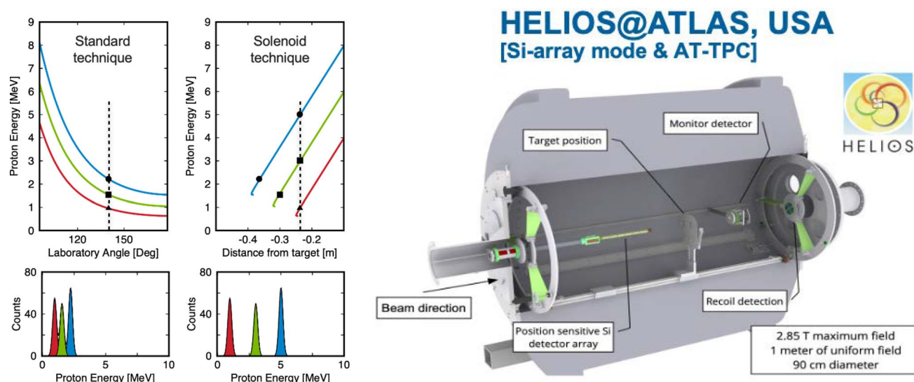
Fig. 53 (left) A comparison between a standard technique to measure light particles in direct reactions in standard kinematics whereby the outgoing protons from a typical ( d,p ) reaction are measured at a fixed angle for three different final states (red, green and blue), and the solenoid technique by which the protons are instead measured at a fixed distance from the reaction target after completing a single cyclotron orbit within the solenoid field. The dashed vertical lines correspond to fixed detector positions either in angle or position. (right) A schematic view of an experimental setup within the HELIOS spectrometer for a typical single-neutron adding ( d,p ) reaction
