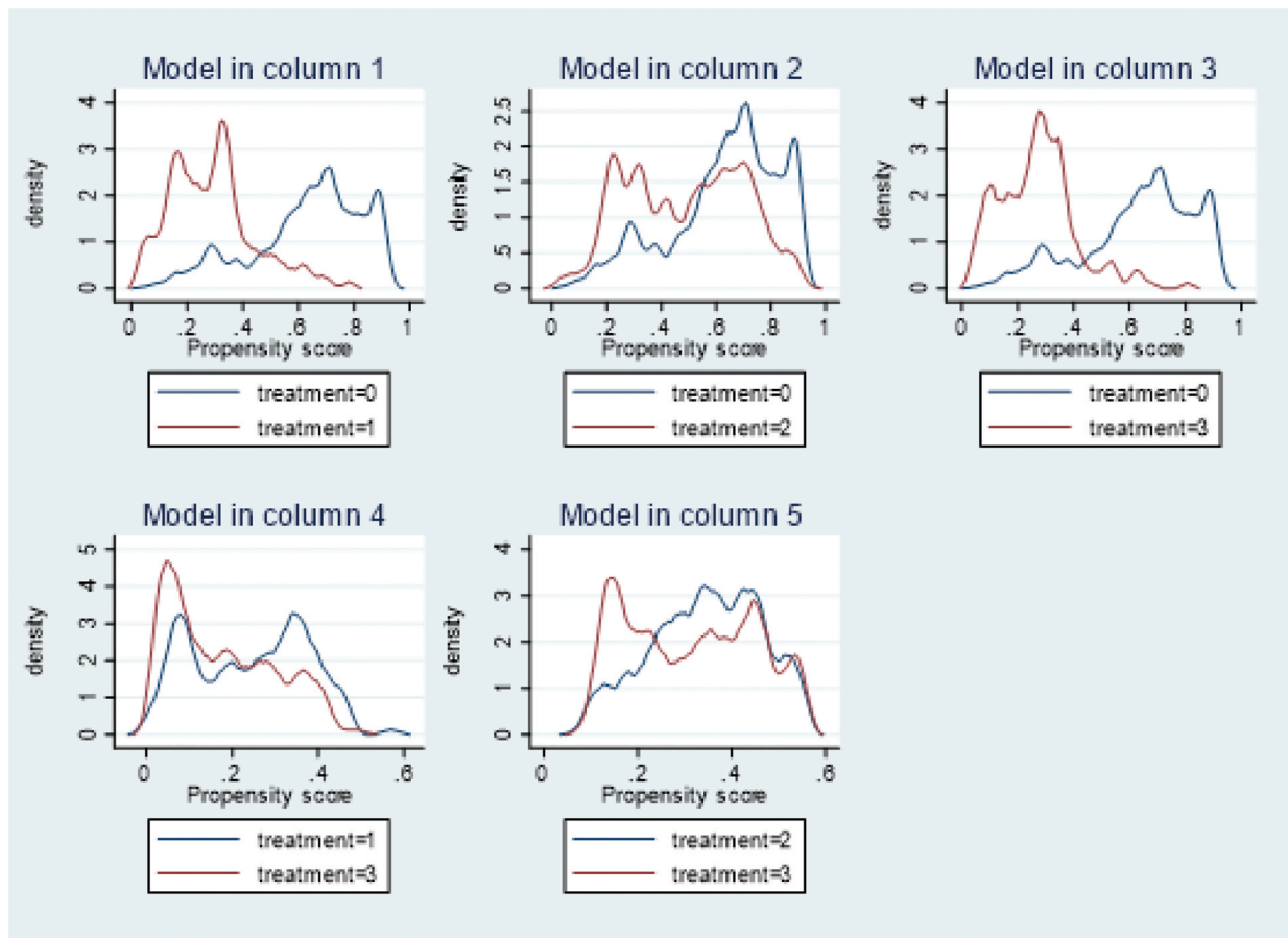
Fig. A1. Checking the overlap assumption for the estimated models in Table 4.
