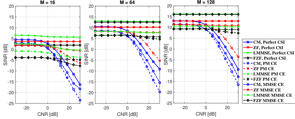
Fig. 1. SINR versus CNR of four detection strategies in the cases of perfect CSI, PM CE and MMSE CE, with K = 10 and different values of M .
