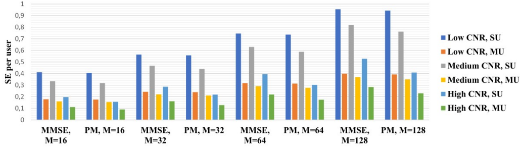
Fig. 2. SE per user lower bounds, in SU and MU scenarios, for increasing values of M , for \text{CNR} = -20 dB (Low CNR), for \text{CNR} = 0 dB (Medium CNR), for \text{CNR} = 10 dB (High CNR), and with PM and MMSE CE techniques.
