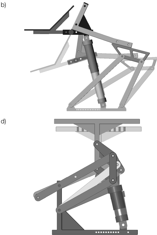
Figure 3 Trajectories of the moving parts a) US Patent US 6,019,380 b) Flex sit-ski c) modified Flex sit-ski d) eight-bar linkage
