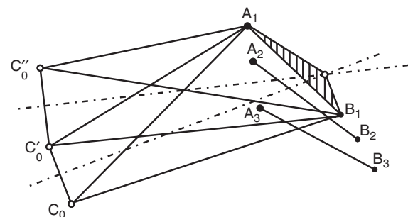
Figure 7 Kinematic inversion
